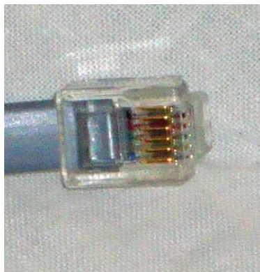
Good crimp Jacket inside plug
