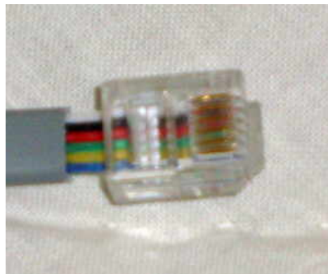
Bad crimp Jacket not inside plug
